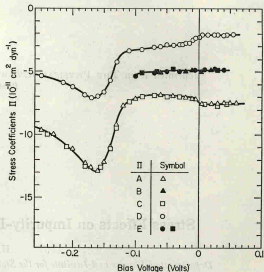
Fig. 2. Stress coefficients for uniaxial compression and hydrostatic pressure for As-doped Ge tunnel junctions as a function of bias voltage at 4.2°K. Note the factor \frac{1}{13} in the definition of the hydrostatic-pressure coefficients B and E .
